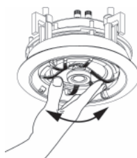
Figure 5. Woofer adjustment.
